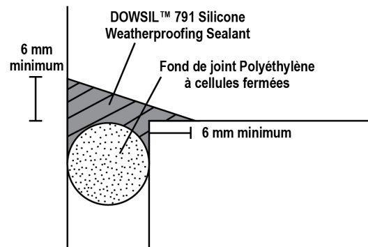
Figure 3: Joint D'angle
